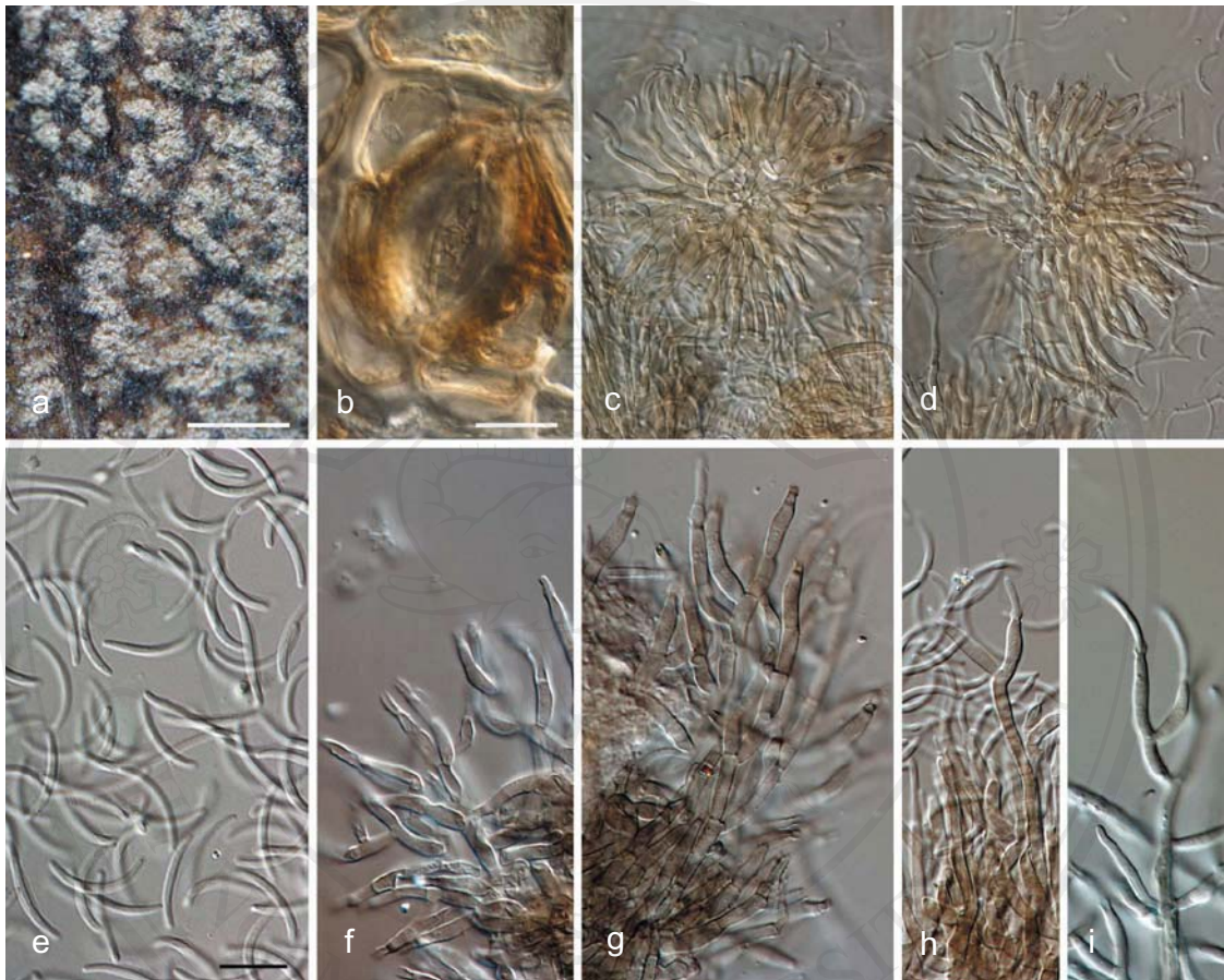
Fig. 6.3 Bagadiella lunata . a. Caespituli on leaf; b. pseudoparenchymatal tissue in substomatal cavity; c, d. rosette of conidiophores; e. conidia; f–i. conidia. — Scale bars: a = 300 \mu\text{m} ; b–d = 30 \mu\text{m} ; e–h = 20 \mu\text{m} , b applies to b–d, e applies to e–i.
