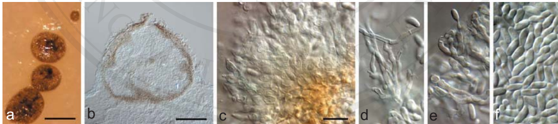
Fig. 6.9 Foliocryphia eucalypti . a. Pycnidia on OA; b. cross section of conidioma; c–e. conidiophores and conidiogenous cells; f. conidia. — Scale bars: a = 450 \mu\text{m} ; b = 100 \mu\text{m} ; c–f = 10 \mu\text{m} .
