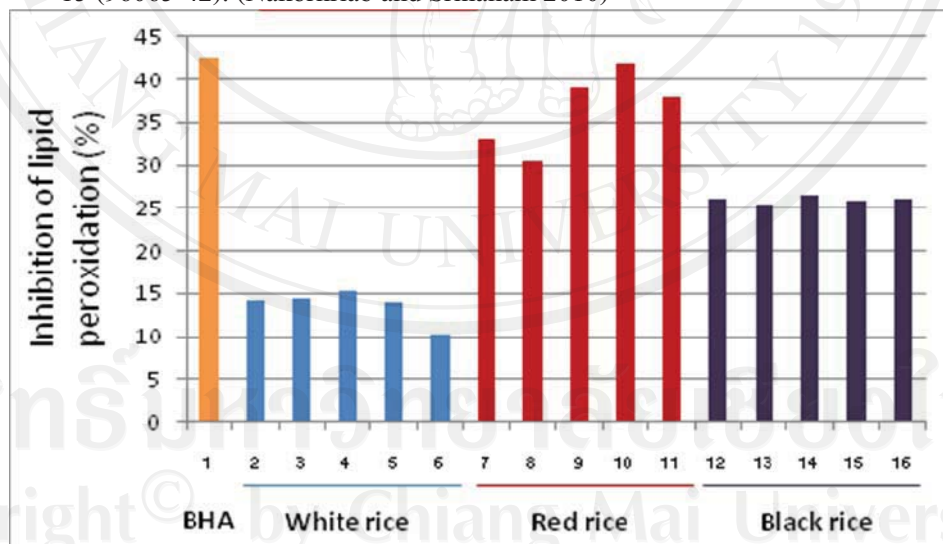
Figure 11 Antioxidative activity of crude extracts of Thai rice bran using thiocyanate method expressed as % inhibition of lipid peroxidation: white rice; 2 (Mali105), 3 (Supun), 4 (Saohai), 5 (Homjun), 6 (Homchaiya), red rice; 7 (3256), 8 (GS18003), 9 (21606), 10 (21699), 11 (5718), black rice; 12 (96041-20), 13 (96051-37), 14 (96004-49), 15 (96023-35) and 16 (96065-42) which compared with BHA (No.1). (Nakornriab and Srihanam 2010)
