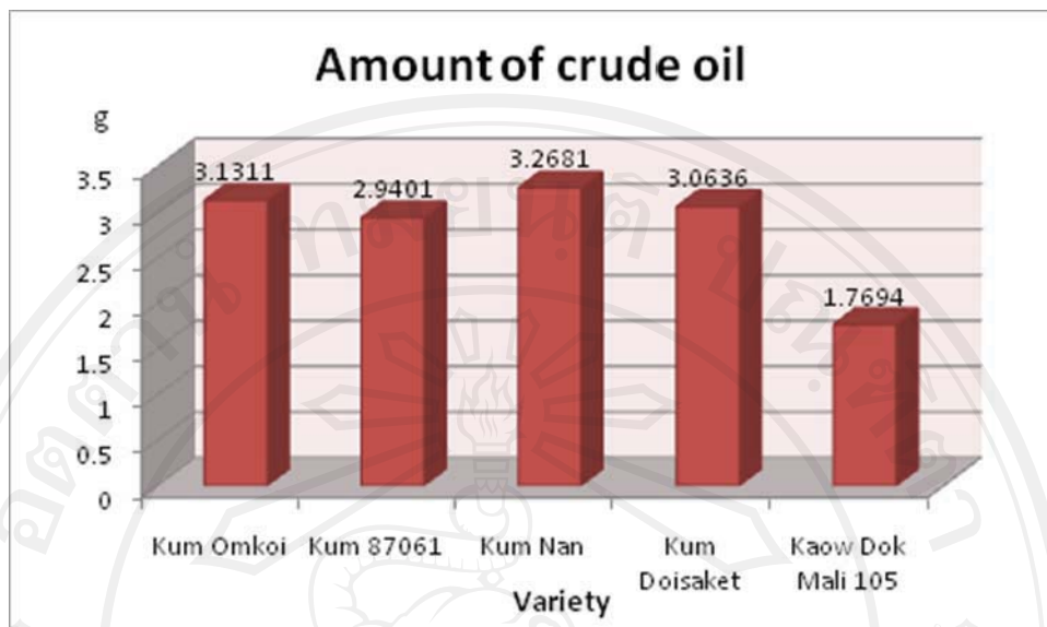
Figure 4 Comparison of the amount of crude oil (g) extracted from bran of various purple glutinous rice cultivars (Kum) and of controlled white rice (Kaow Dok Mali 105) (Karladee et al. , 2003)
