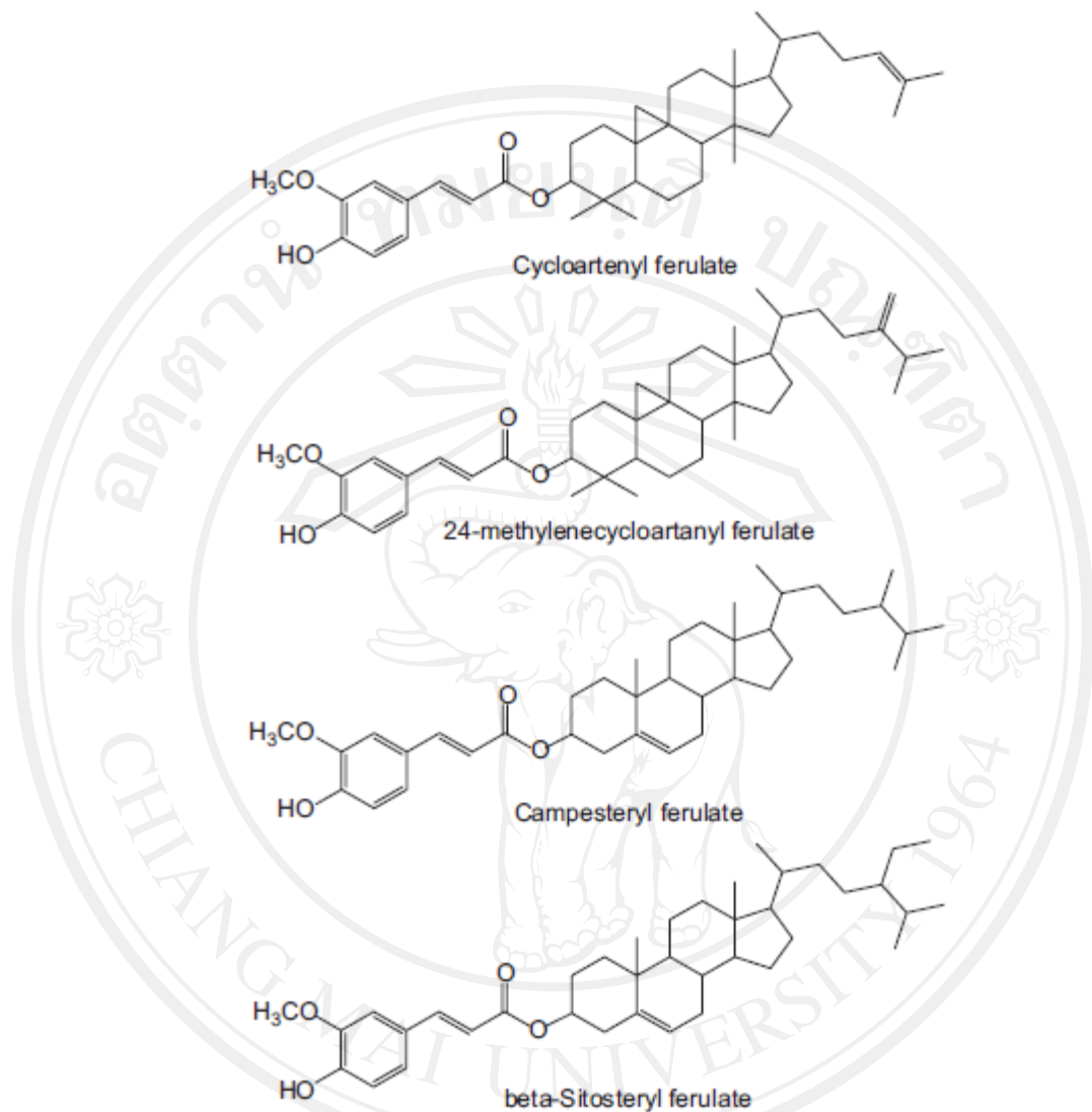
Figure 8 The 4 major chemical structure forms of ferulic acid (cycloartenyl ferulate, 24-methylene cycloartenyl ferulate, campesteryl ferulate and beta-sitosteryl ferulate) (Chotimakorn and Ushio, 2008)
