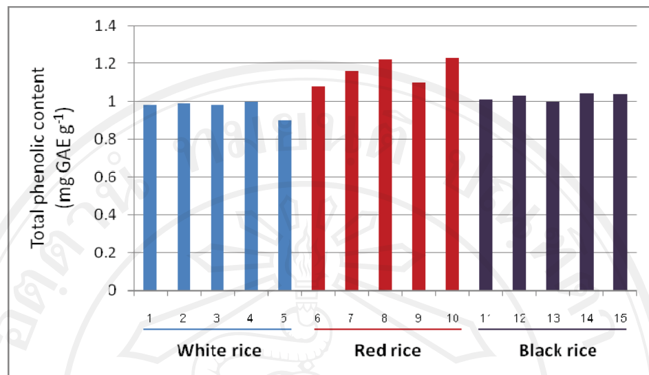
Figure 10 Total phenolic content of Thai rice bran extracts measured by the Folin-Ciocalteu method expressed as mg GAE/g: white rice; 1 (Mali105), 2 (Supun), 3 (Saohai), 4 (Homjun), 5 (Homchaiya), red rice; 6 (3256), 7 (GS18003), 8 (21606), 9 (21699), 10 (5718), black rice; 11 (96041-20), 12 (96051-37), 13 (96004-49), 14 (96023-35) and 15 (96065-42). (Nakornriab and Srihanam 2010)
