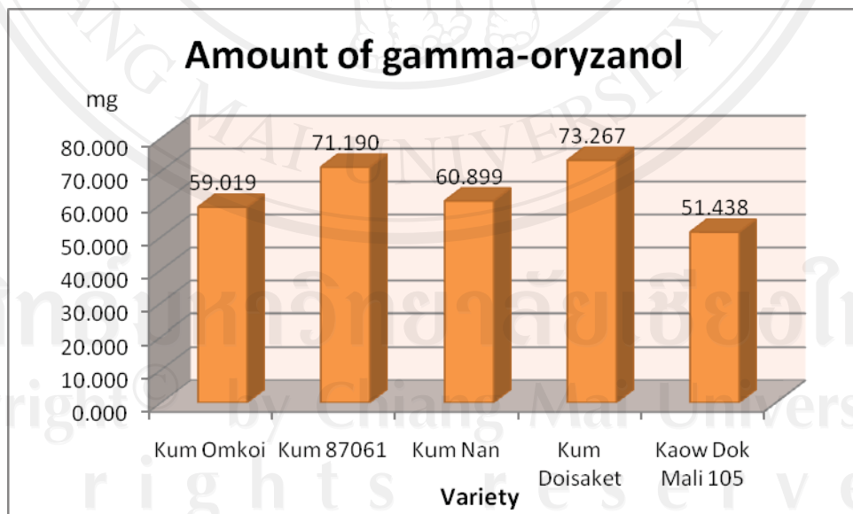
Figure 7 Comparison of the amount of \gamma - Oryzanol in crude oil (mg) extracted from brown rice of various purple glutinous rice cultivars (Kum) and of controlled white rice (Kaow Dok Mali 105) (Karladee et al. , 2003)
