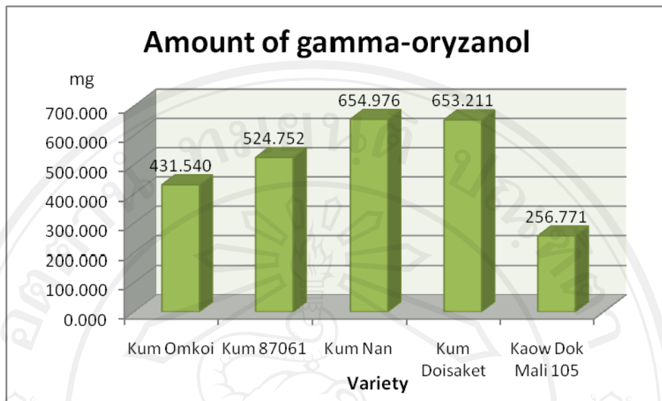
Figure 6 Comparison of the amount of \gamma - Oryzanol in crude oil (mg) extracted from bran of various purple glutinous rice cultivars (Kum) and of controlled white rice (Kaow Dok Mali 105) (Karladee et al. , 2003)
