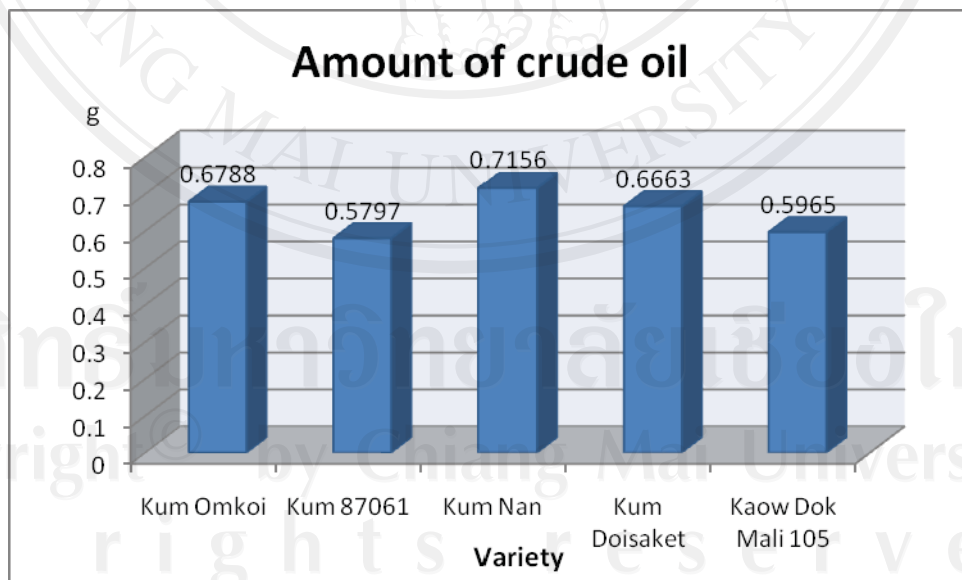
Figure 5 Comparison of the amount of crude oil (g) extracted from brown rice of various purple glutinous rice cultivars (Kum) and of controlled white rice (Kaow Dok Mali 105) (Karladee et al. , 2003)
