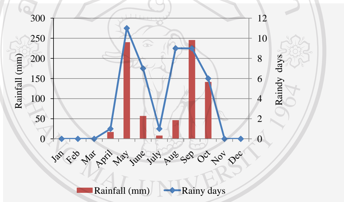
Figure 4.1 Distribution of rainfall (mm) and rainy days in Kyaukse township
