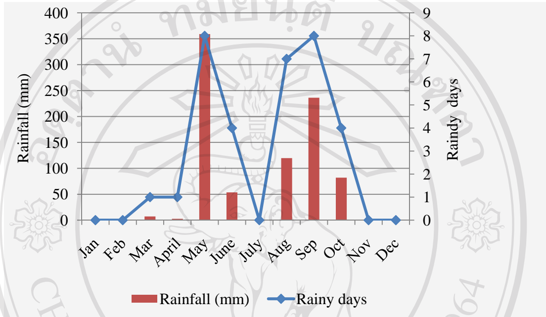
Figure 4.2 Distribution of rainfall (mm) and rainy days in Myittha township
